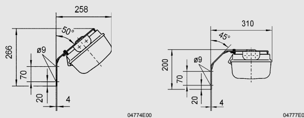
Wall-mounting bracket 50°
