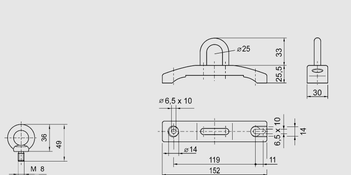
Ring bolt
