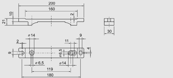
Ceiling mounting bracket
