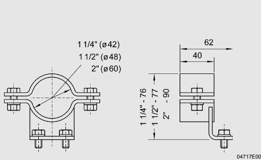
Pipe clamp
