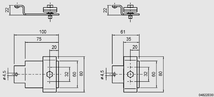
Mounting set grid cable rack
