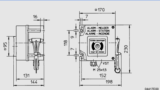
8146/5052-C796, -C797 and -C814 Alarm stations
