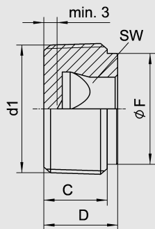
Stopping plug, 8294/111, NPT, hexagon socket
